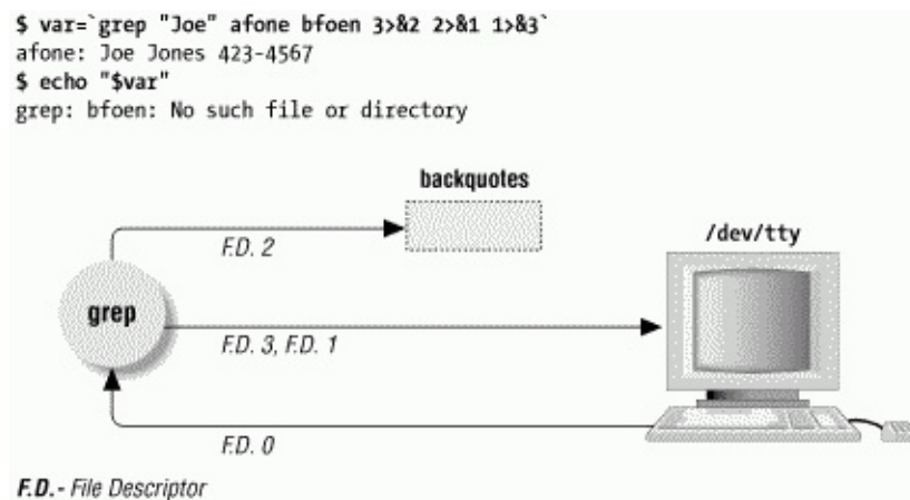
Figure 36-6. File descriptors after 3>&2 2>&1 1>&3 redirection
