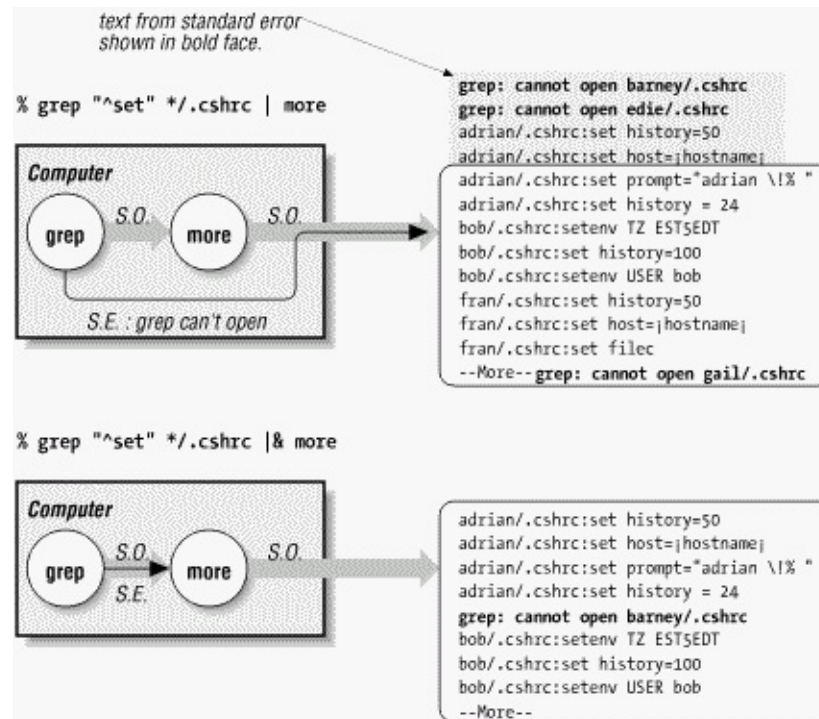
Figure 43-1. Standard error bypassing pipe, going through pipe
