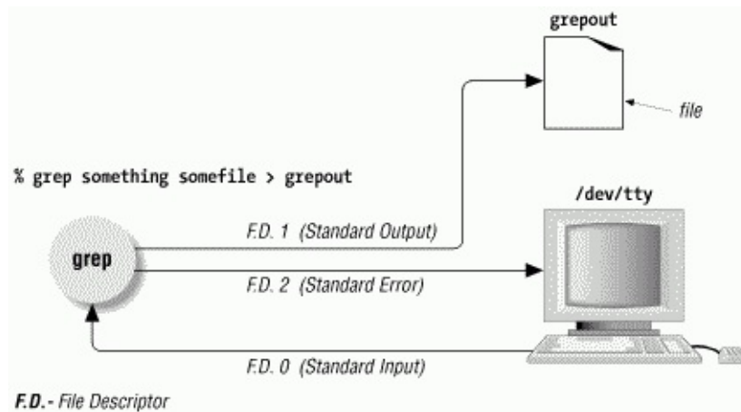
Figure 36-2. Standard output redirected to a file
