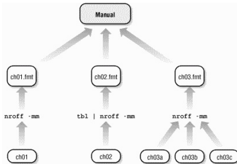
Figure 11-1. What Makefile describes: Files and commands to make manual
