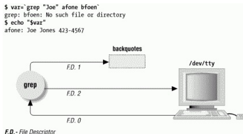
Figure 36-4. File descriptors after 3>&2 redirection
