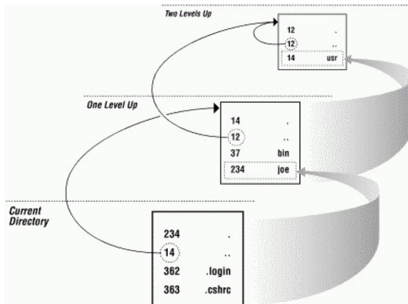
Figure 31-2. Finding the current directory name
