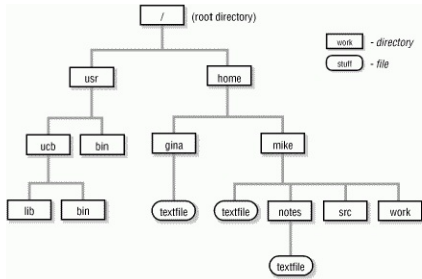
Figure 1-4. Part of a Unix filesystem tree
