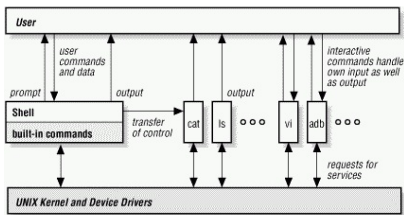
Figure 1-1. Relationship of kernel, shell, utilities, and applications
