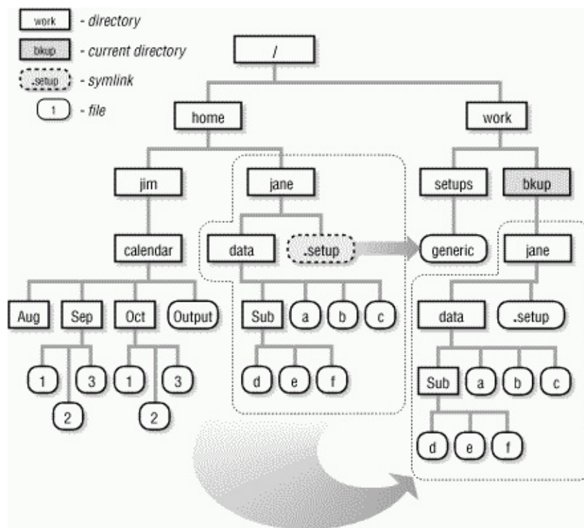
Figure 10-1. Copying /home/jane to /work/bkup with tar
