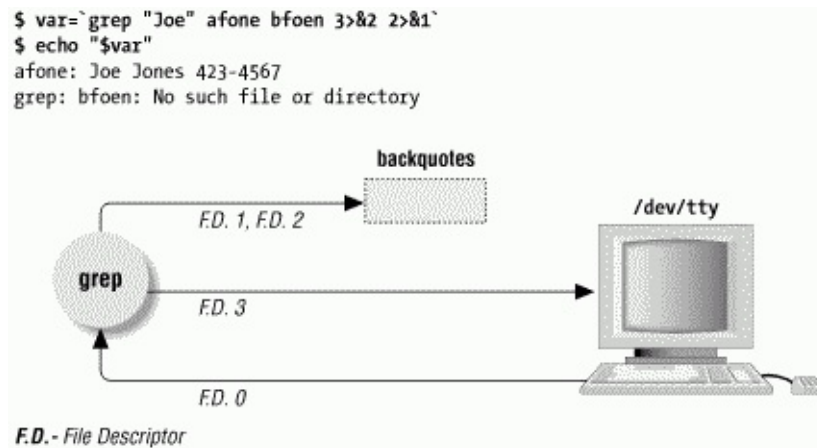
Figure 36-5. File descriptors after 3>&2 2>&1 redirection
